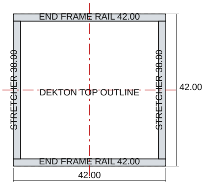
PLAN — BASE FRAME, TOP REMOVED
